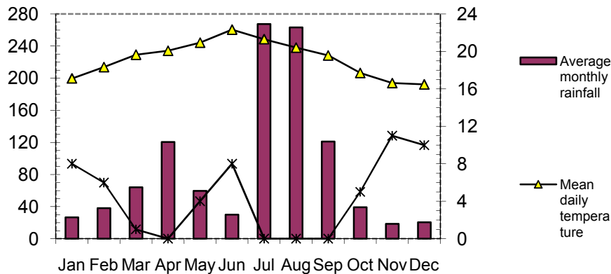
Figure 1: Average monthly rainfall, mean daily temperature and number of years that had less than 14.7mm monthly rainfall out of 16 years of data from Combolcha meteorological station (1985-2000).
